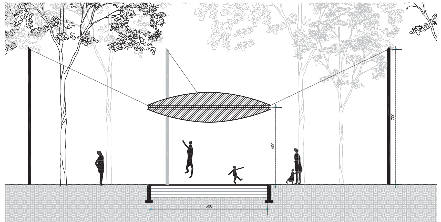
section . 1/100
